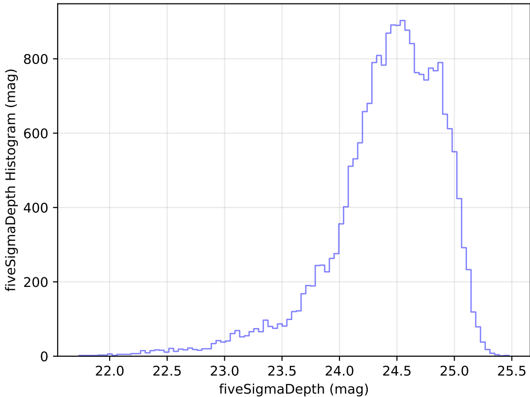
weather_cloudso10v3.4_10yrs Yr 1 g band: fiveSigmaDepth Histogram
