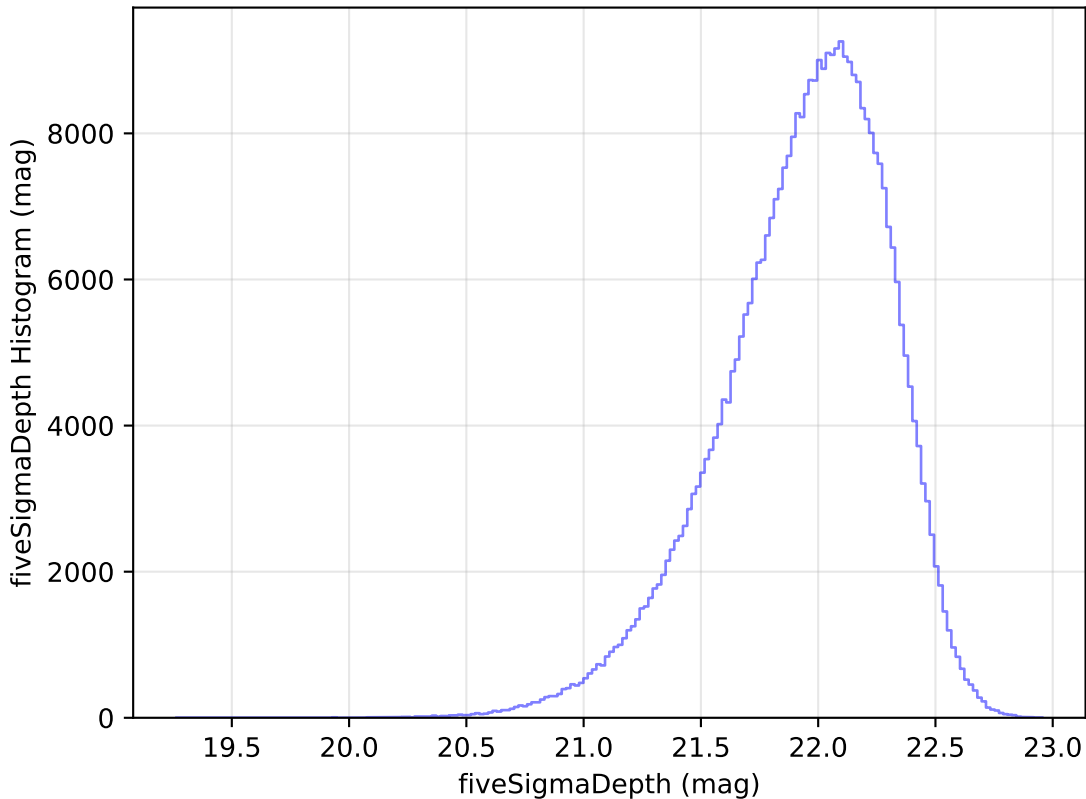
weather_cloudso10v3.4_10yrs WFD y band: fiveSigmaDepth Histogram
