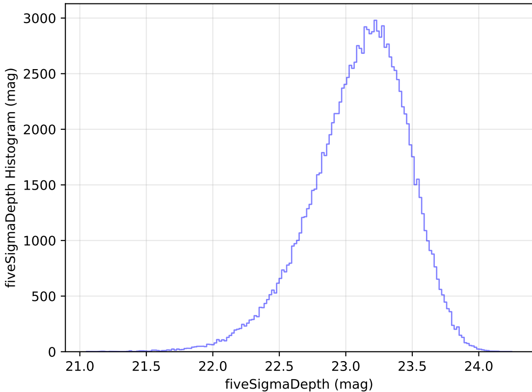
weather_cloudso10v3.4_10yrs WFD u band: fiveSigmaDepth Histogram
