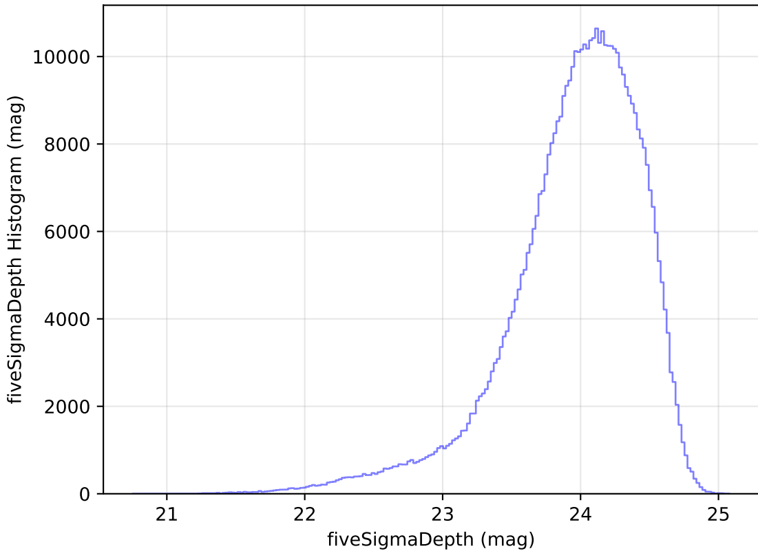
weather_cloudso10v3.4_10yrs WFD r band: fiveSigmaDepth Histogram
