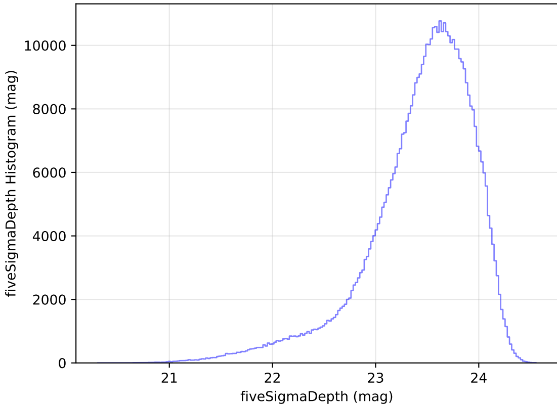
weather_cloudso10v3.4_10yrs WFD i band: fiveSigmaDepth Histogram
