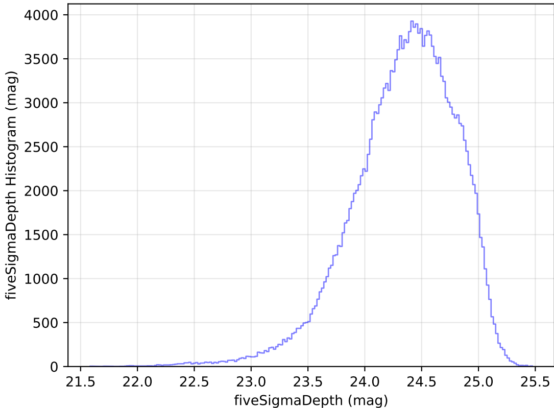
weather_cloudso10v3.4_10yrs WFD g band: fiveSigmaDepth Histogram
