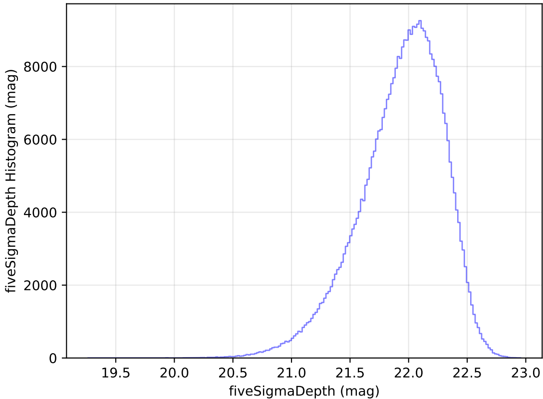
weather_cloudso10v3.4_10yrs All sky y band: fiveSigmaDepth Histogram
