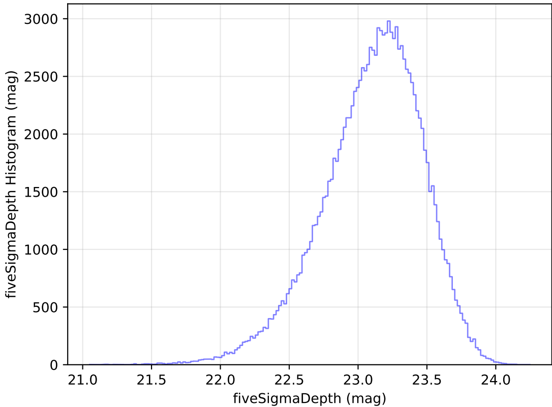
weather_cloudso10v3.4_10yrs All sky u band: fiveSigmaDepth Histogram
