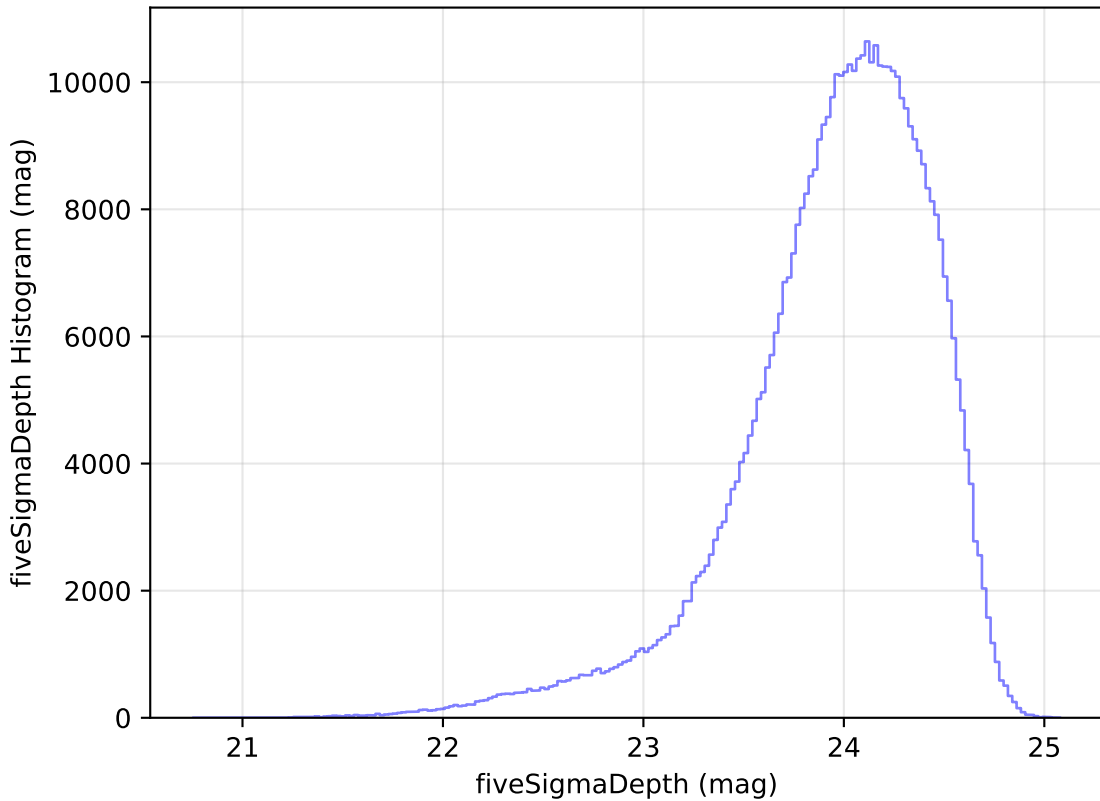
weather_cloudso10v3.4_10yrs All sky r band: fiveSigmaDepth Histogram
