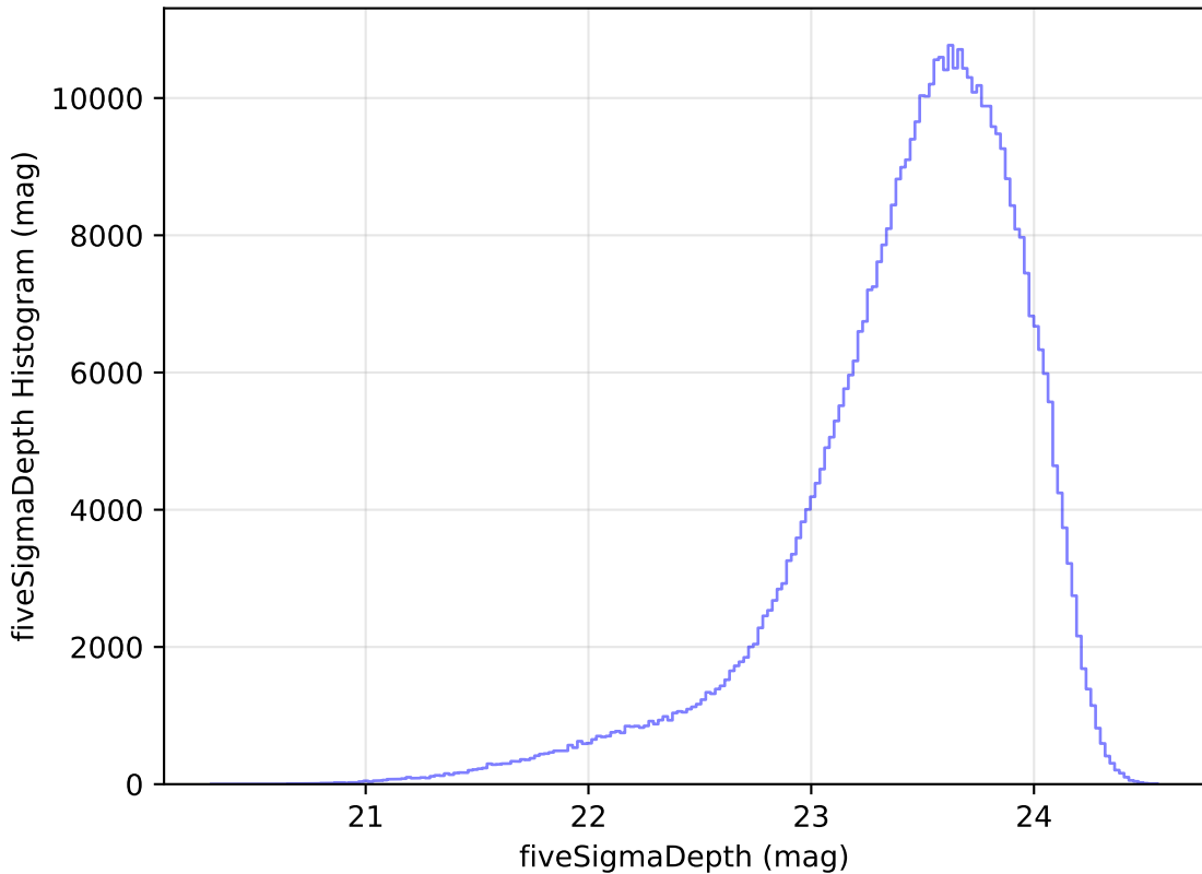
weather_cloudso10v3.4_10yrs All sky i band: fiveSigmaDepth Histogram
