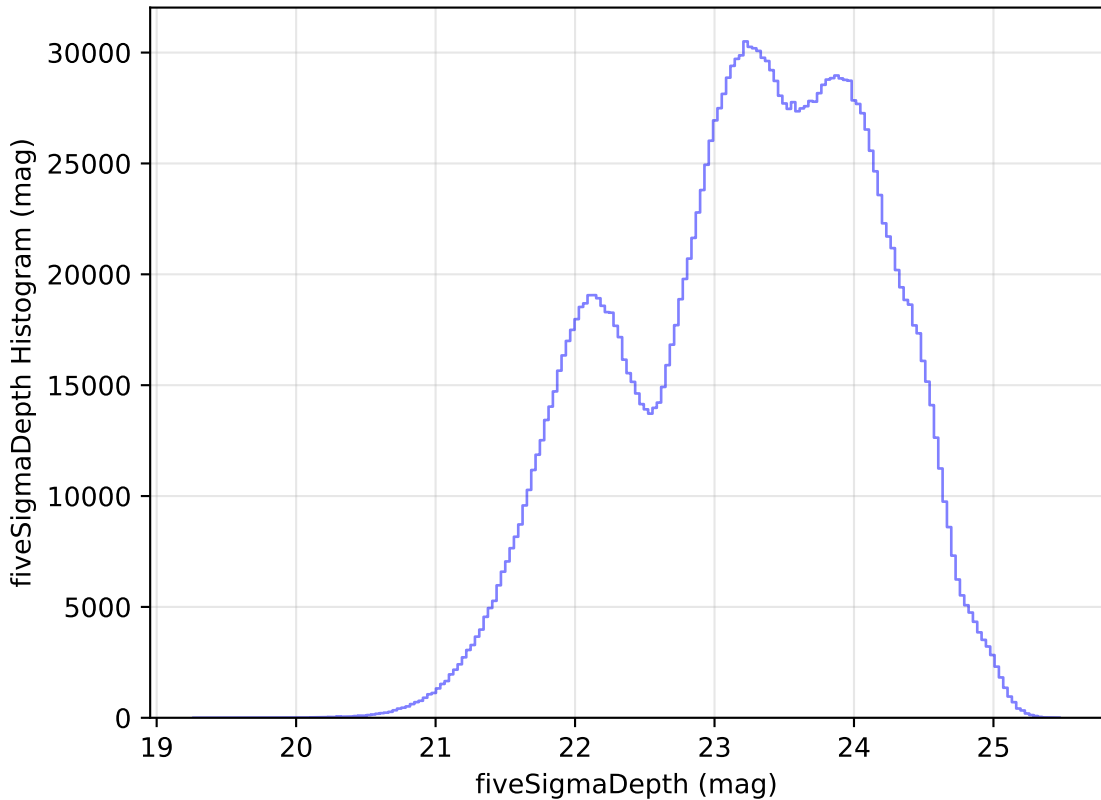
weather_cloudso10v3.4_10yrs All sky all bands: fiveSigmaDepth Histogram
