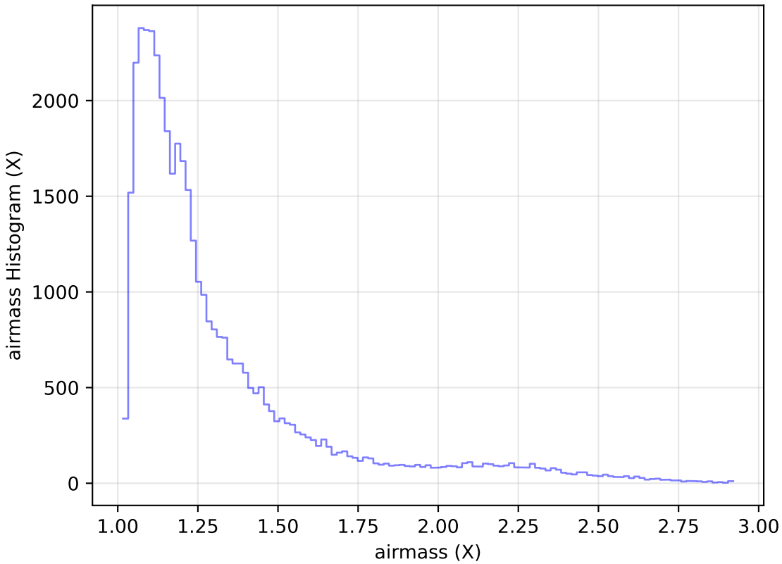
weather_cloudso10v3.4_10yrs Yr 1 z band: airmass Histogram
