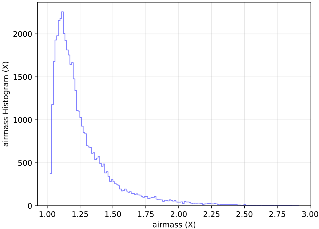
weather_cloudso10v3.4_10yrs Yr 1 y band: airmass Histogram
