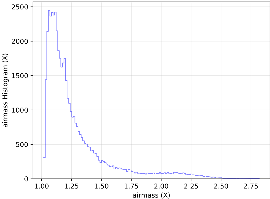
weather_cloudso10v3.4_10yrs Yr 1 r band: airmass Histogram
