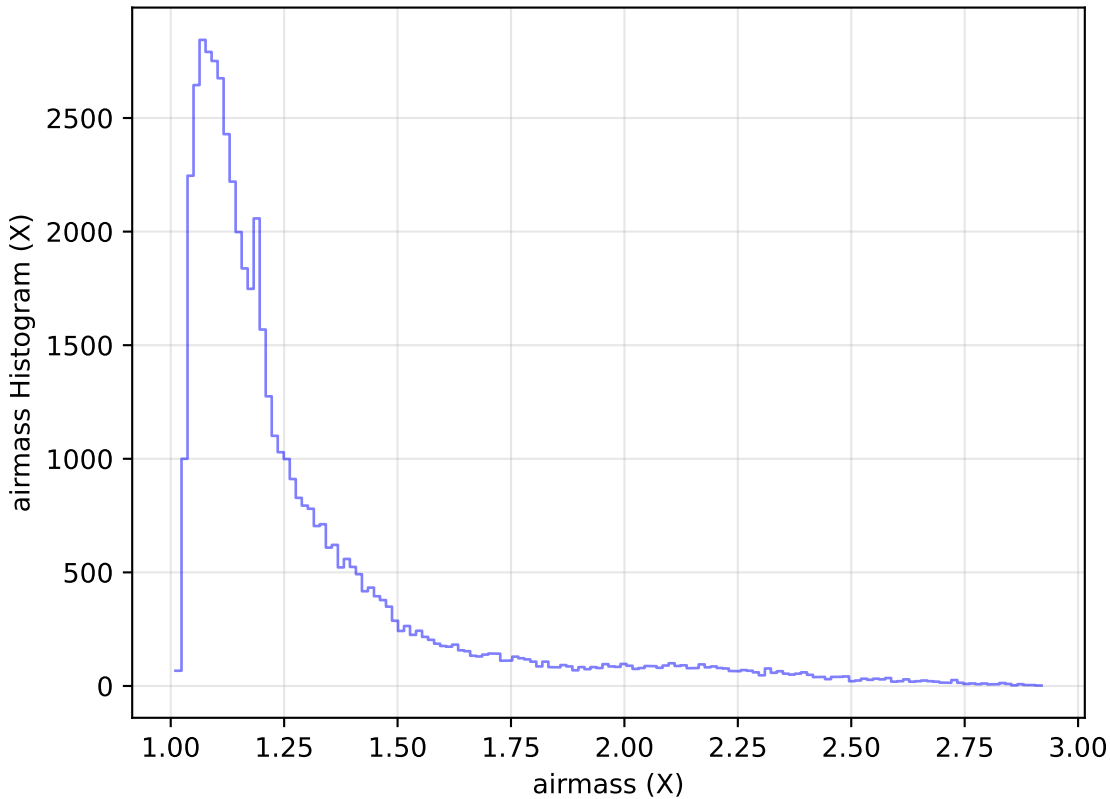
weather_cloudso10v3.4_10yrs Yr 1 i band: airmass Histogram
