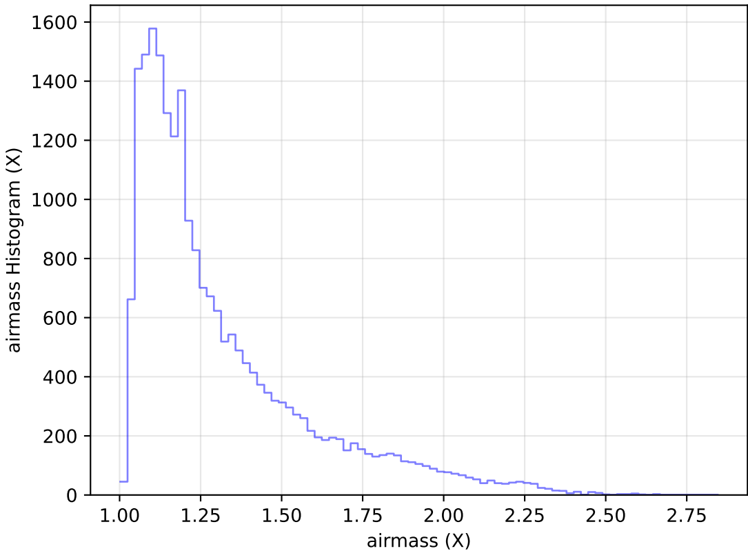
weather_cloudso10v3.4_10yrs Yr 1 g band: airmass Histogram
