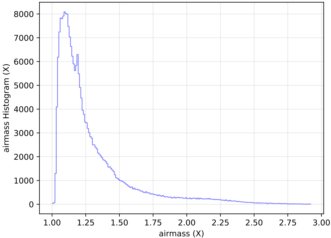
weather_cloudso10v3.4_10yrs Yr 1 all bands: airmass Histogram
