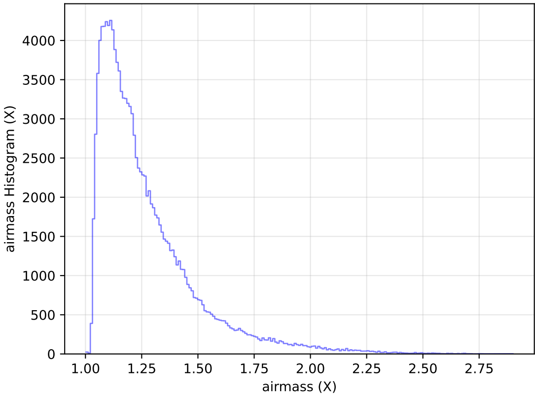
weather_cloudso10v3.4_10yrs WFD u band: airmass Histogram
