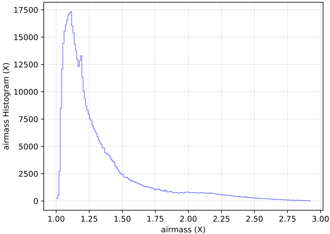
weather_cloudso10v3.4_10yrs WFD i band: airmass Histogram
