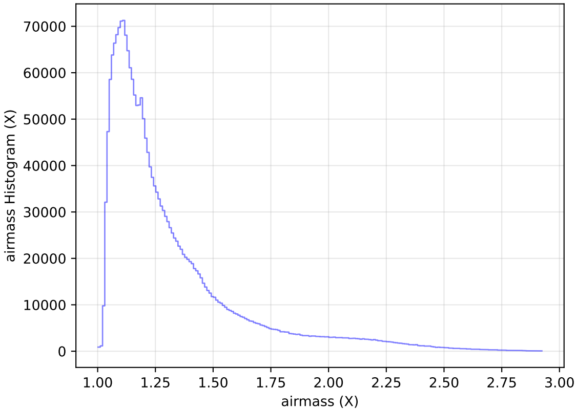
weather_cloudso10v3.4_10yrs WFD all bands: airmass Histogram
