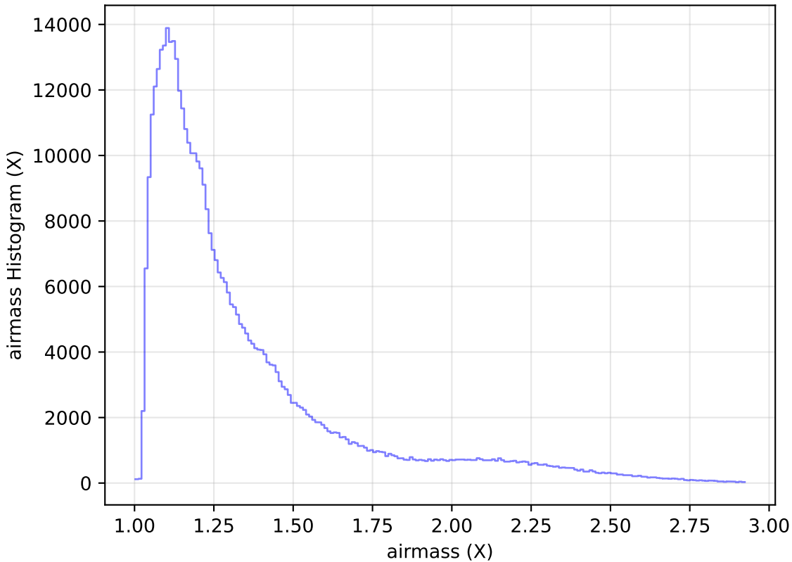
weather_cloudso10v3.4_10yrs All sky z band: airmass Histogram
