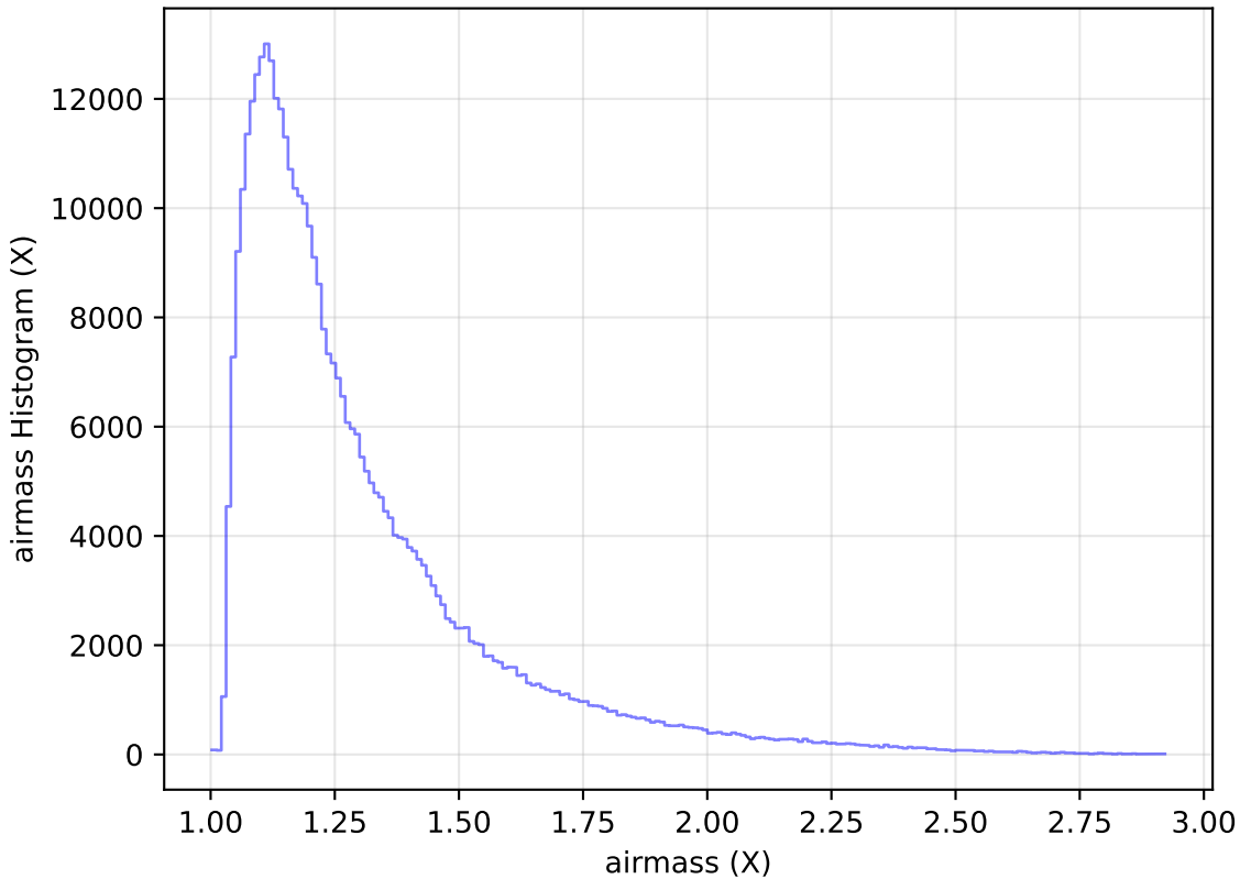
weather_cloudso10v3.4_10yrs All sky y band: airmass Histogram
