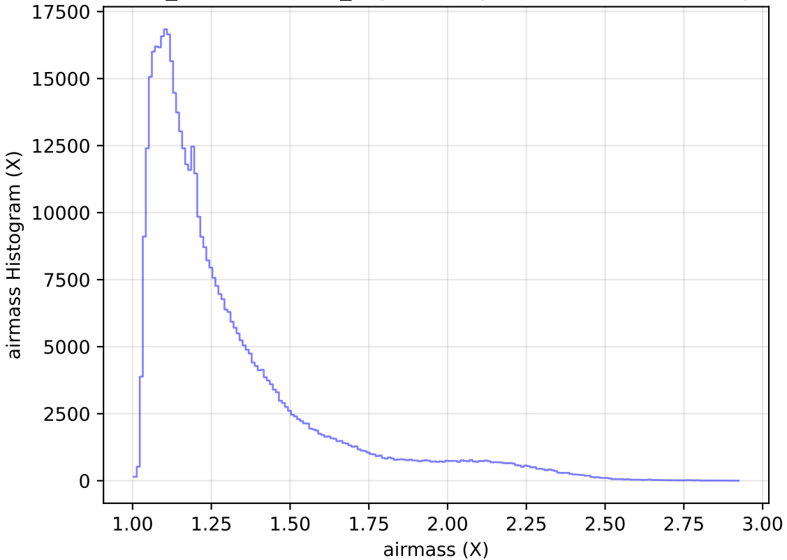
weather_cloudso10v3.4_10yrs All sky r band: airmass Histogram
