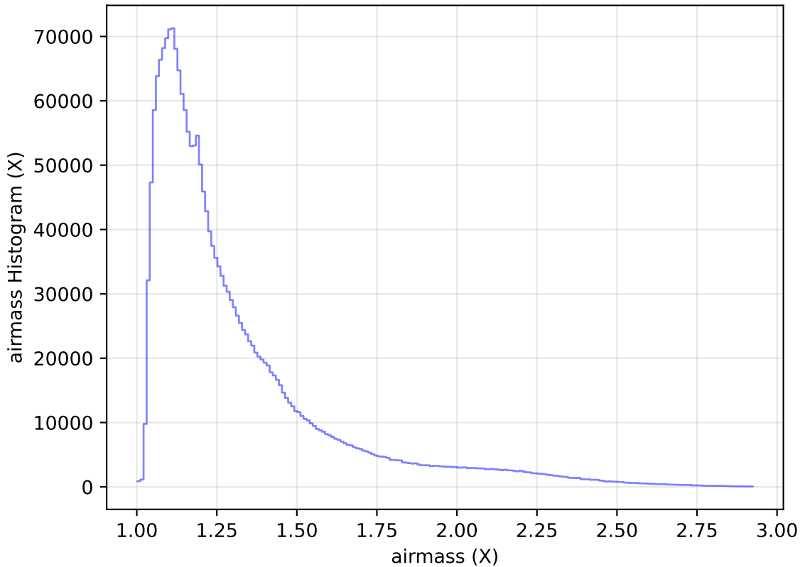
weather_cloudso10v3.4_10yrs All sky all bands: airmass Histogram
