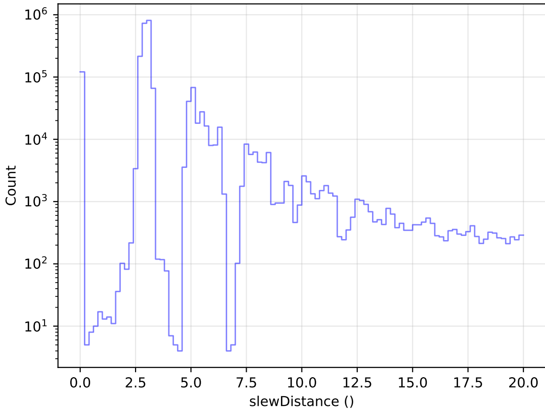
weather_cloudso10v3.4_10yrs All visits: Zoom Slew Distance Histogram
