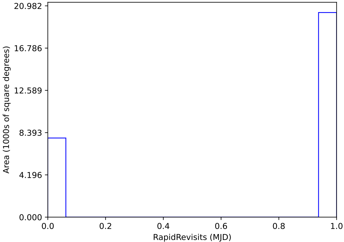
weather_cloudso10v3.4_10yrs All sky: RapidRevisits
