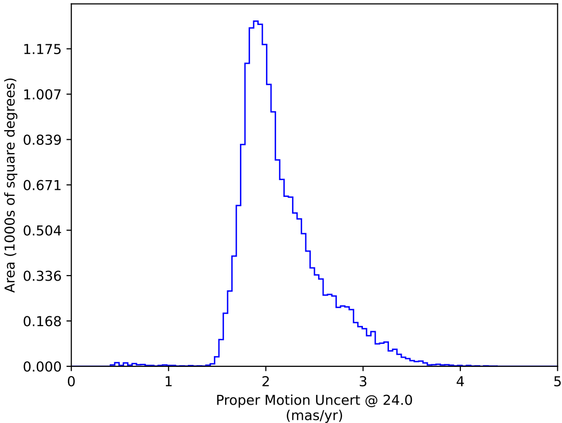
weather_cloudso10v3.4_10yrs WFD: Proper Motion Uncert @ 24.0
