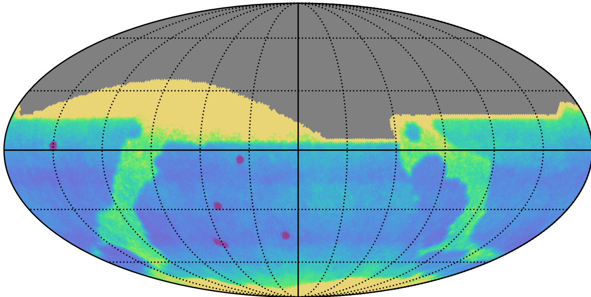
weather_cloudso10v3.4_10yrs All sky: Proper Motion Uncert @ 24.0
