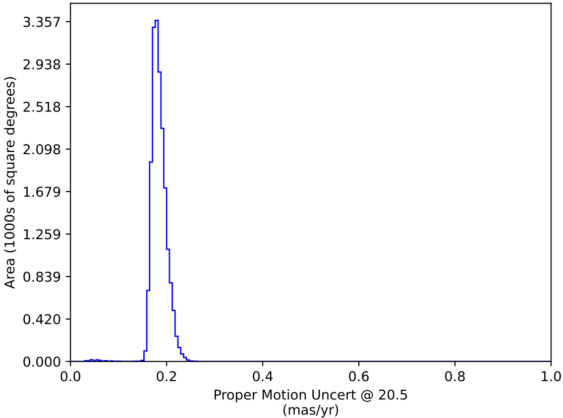
weather_cloudso10v3.4_10yrs WFD: Proper Motion Uncert @ 20.5
