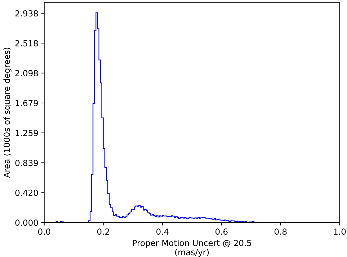
weather_cloudso10v3.4_10yrs All sky: Proper Motion Uncert @ 20.5
