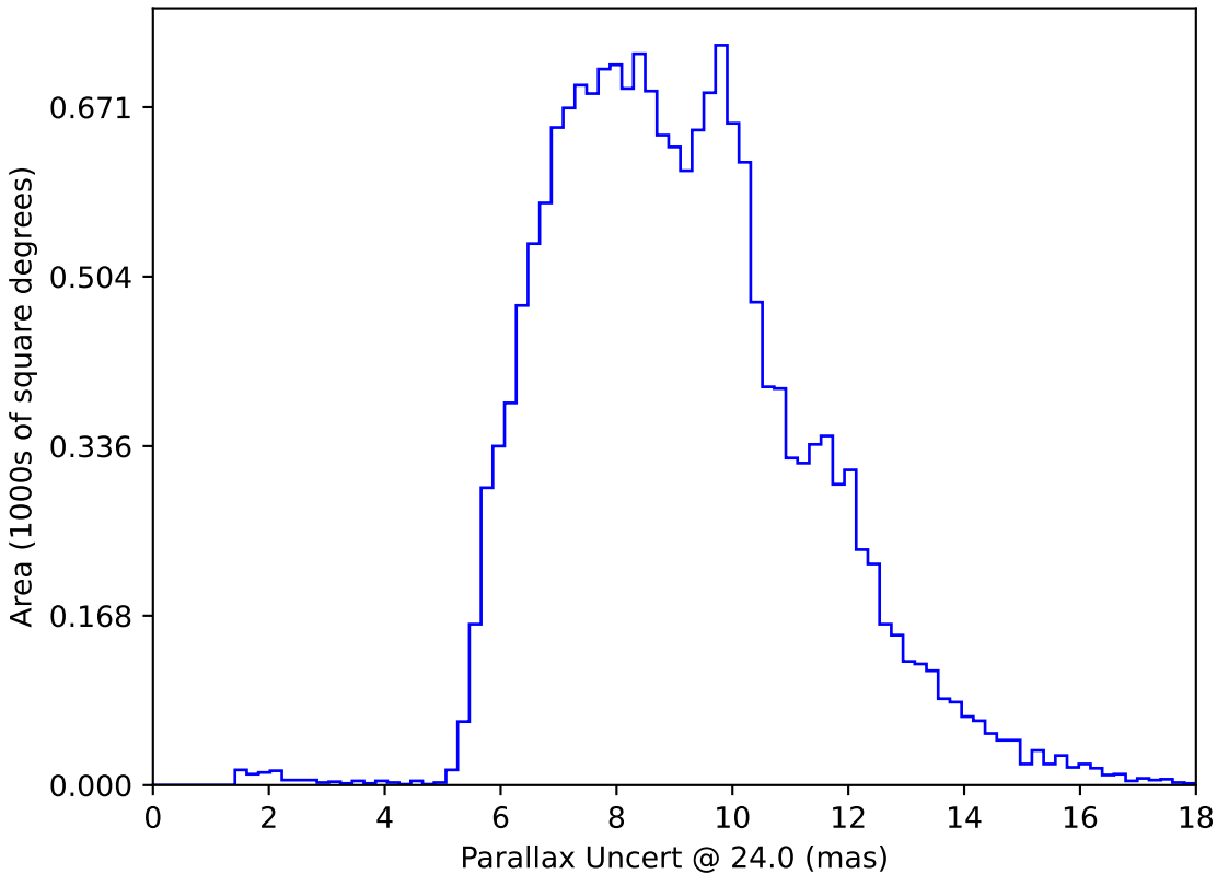
weather_cloudso10v3.4_10yrs WFD: Parallax Uncert @ 24.0
