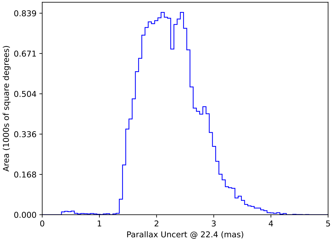
weather_cloudso10v3.4_10yrs WFD: Parallax Uncert @ 22.4
