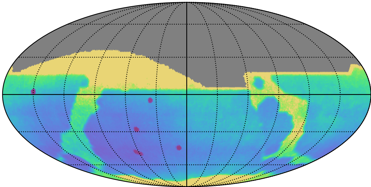
weather_cloudso10v3.4_10yrs All sky: Parallax Uncert @ 22.4
