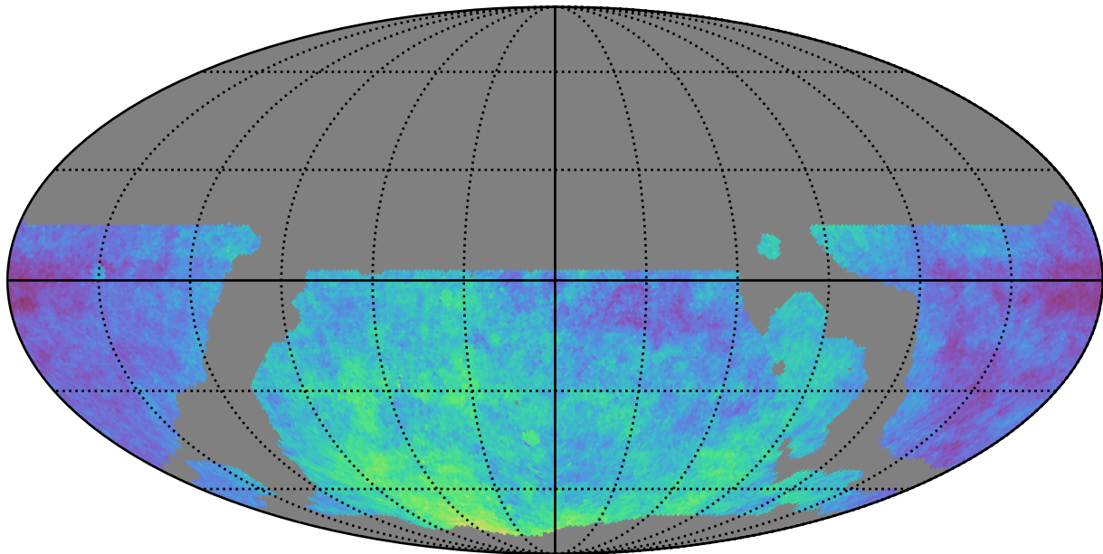
weather_cloudso10v3.4_10yrs WFD: Parallax Coverage @ 24.0
