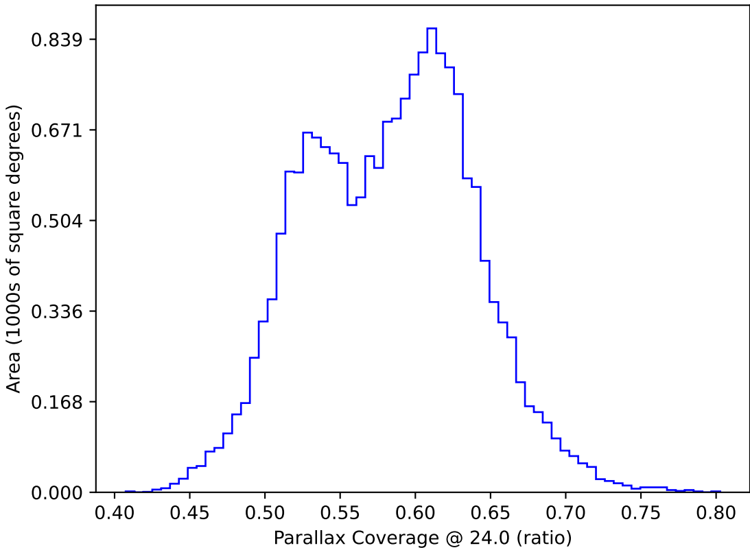
weather_cloudso10v3.4_10yrs WFD: Parallax Coverage @ 24.0
