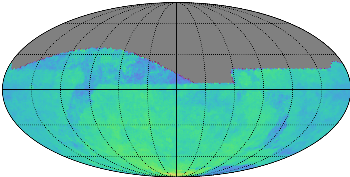
weather_cloudso10v3.4_10yrs All sky: Parallax Coverage @ 24.0
