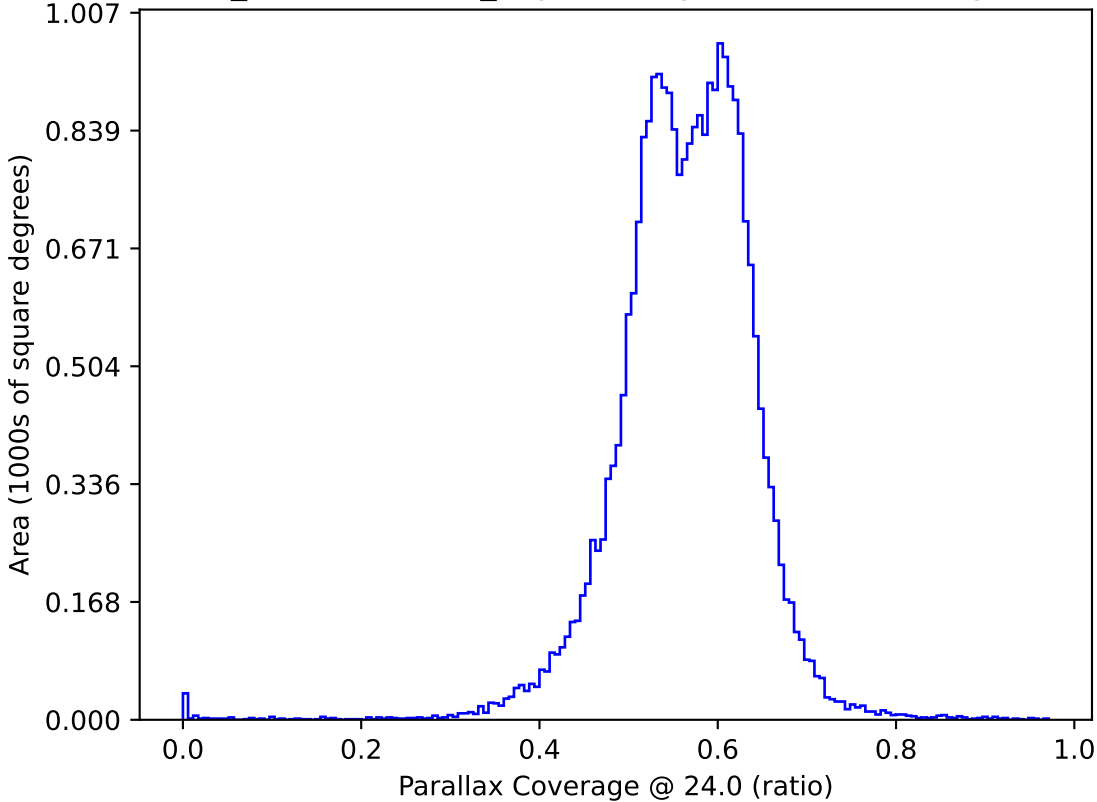
weather_cloudso10v3.4_10yrs All sky: Parallax Coverage @ 24.0
