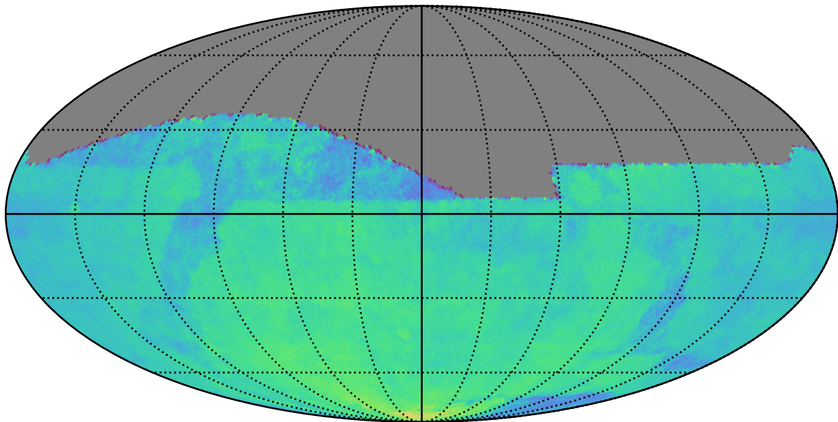
weather_cloudso10v3.4_10yrs All sky: Parallax Coverage @ 22.4
