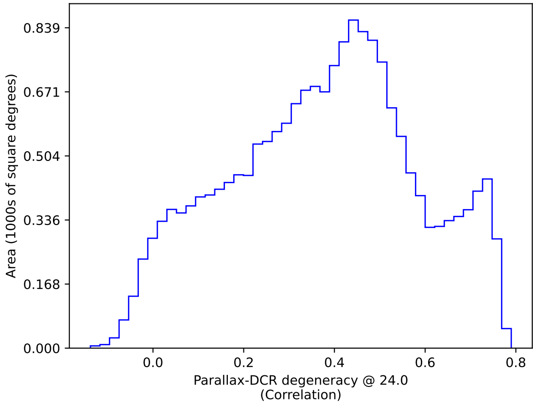
weather_cloudso10v3.4_10yrs WFD: Parallax-DCR degeneracy @ 24.0
