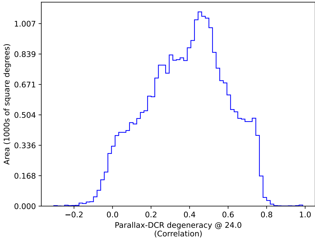
weather_cloudso10v3.4_10yrs All sky: Parallax-DCR degeneracy @ 24.0
