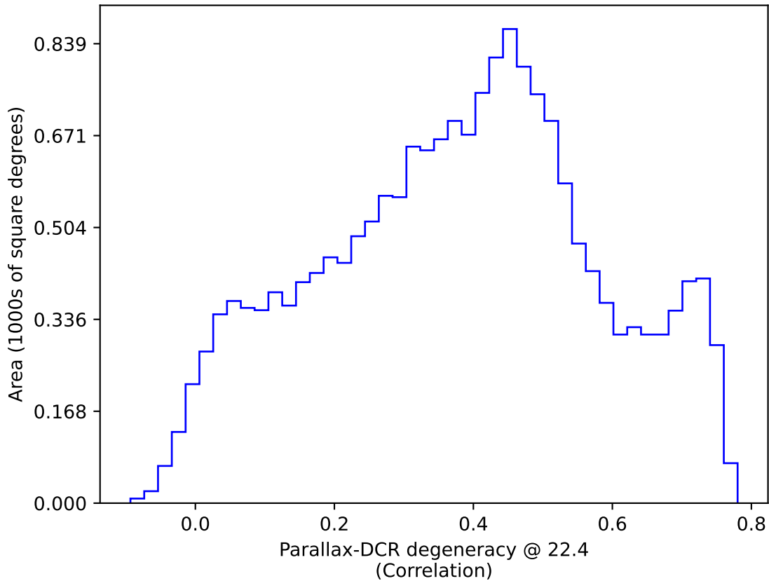
weather_cloudso10v3.4_10yrs WFD: Parallax-DCR degeneracy @ 22.4
