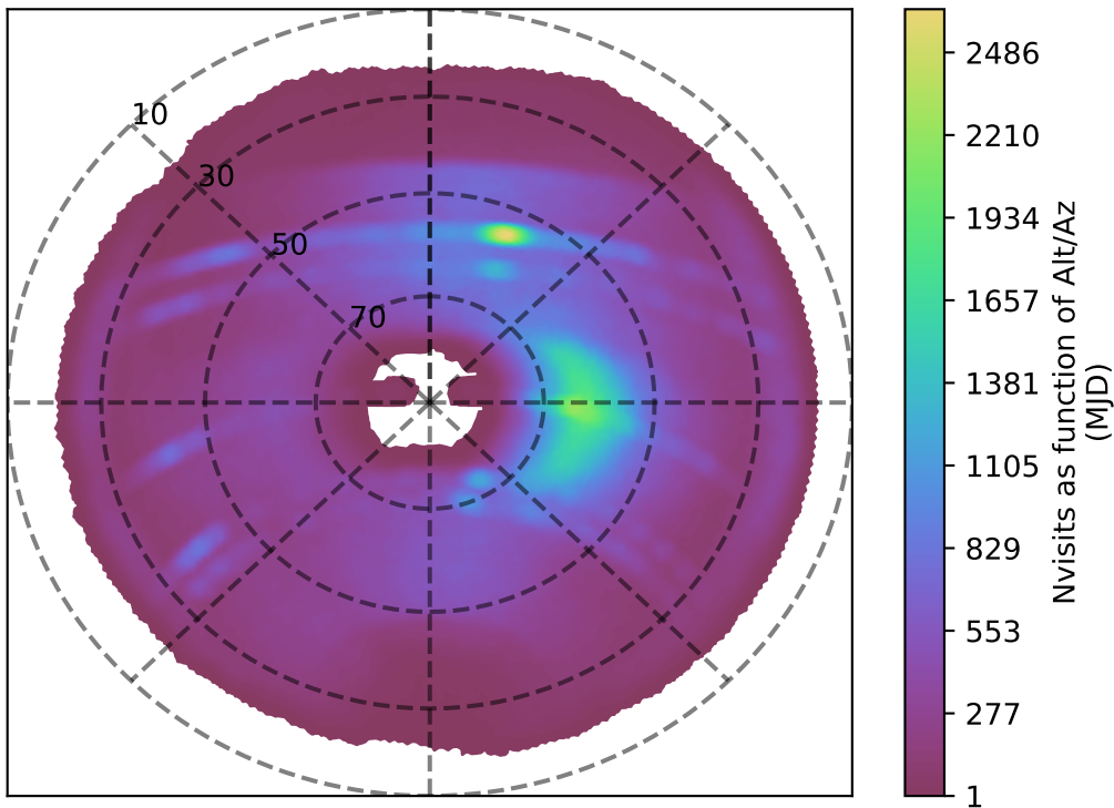
weather_cloudso10v3.4_10yrs z band: Nvisits as function of Alt/Az
