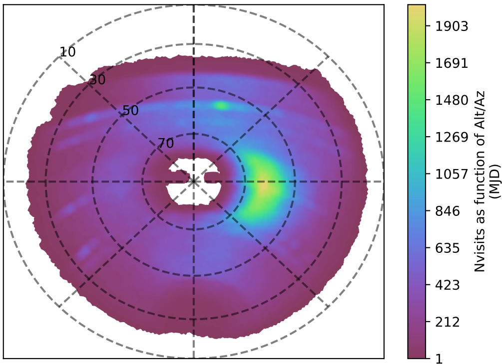
weather_cloudso10v3.4_10yrs y band: Nvisits as function of Alt/Az
