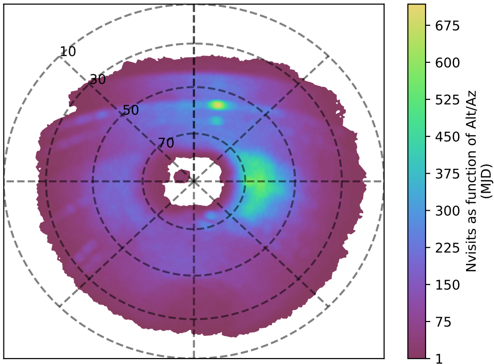
weather_cloudso10v3.4_10yrs u band: Nvisits as function of Alt/Az
