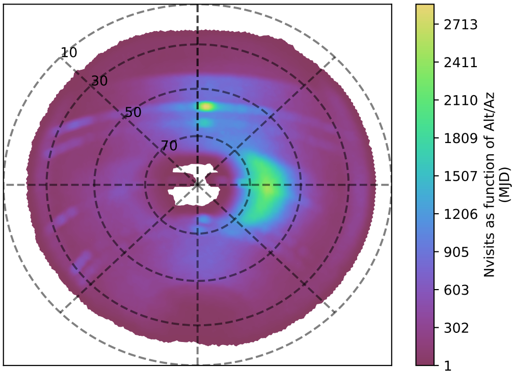
weather_cloudso10v3.4_10yrs i band: Nvisits as function of Alt/Az
