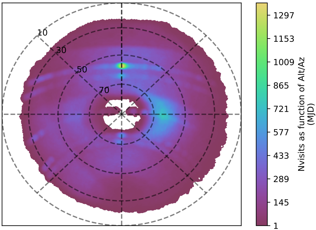
weather_cloudso10v3.4_10yrs g band: Nvisits as function of Alt/Az
