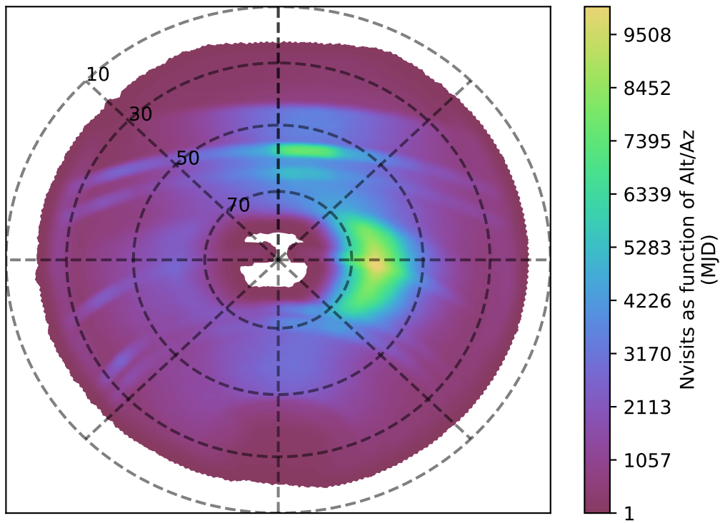
weather_cloudso10v3.4_10yrs all bands: Nvisits as function of Alt/Az
