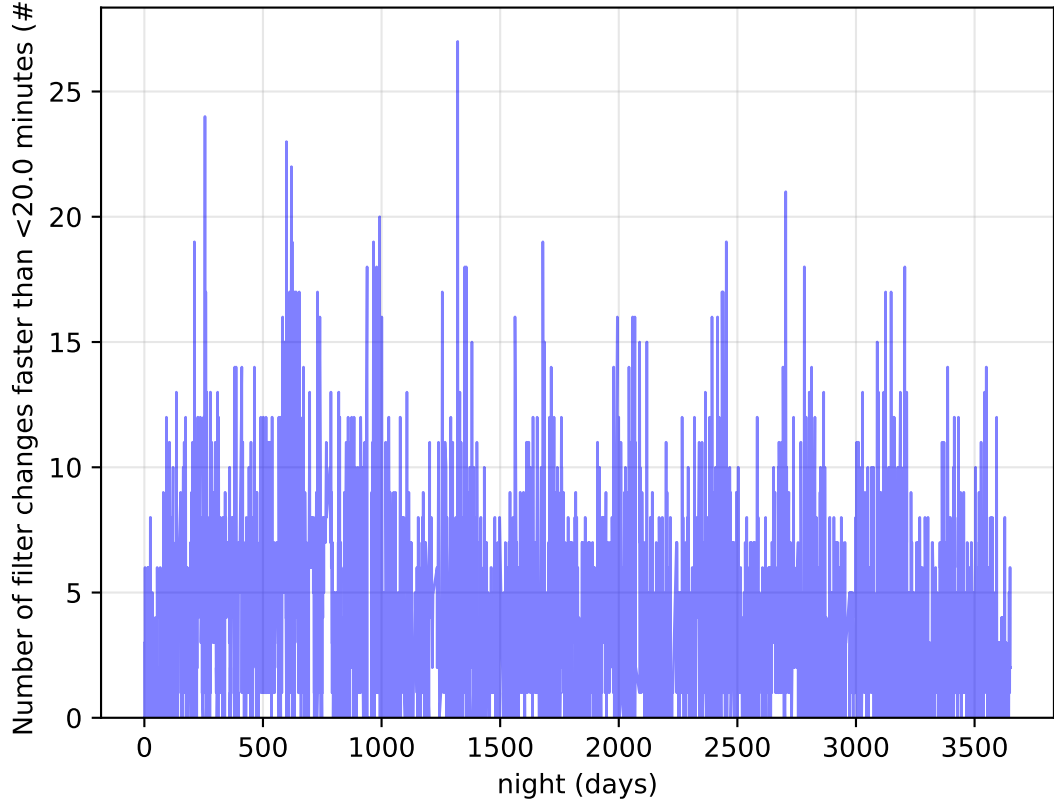
weather_cloudso10v3.4_10yrs Per Night: Number of filter changes faster than <20.0 minutes
