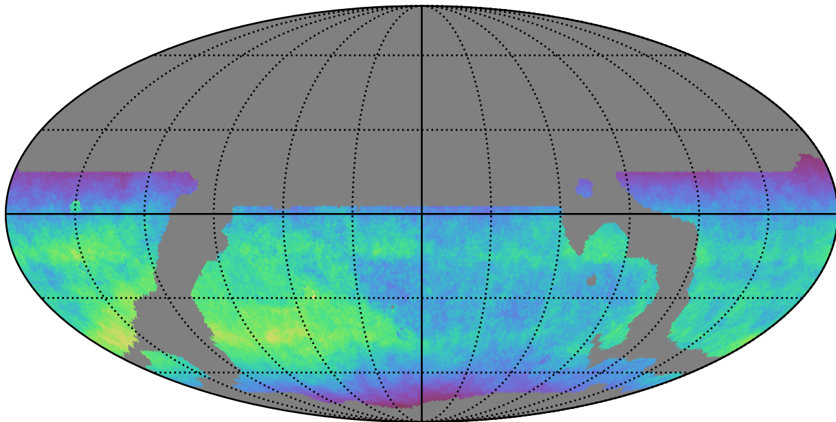
weather_cloudso10v3.4_10yrs WFD z band: Normalized Teff
