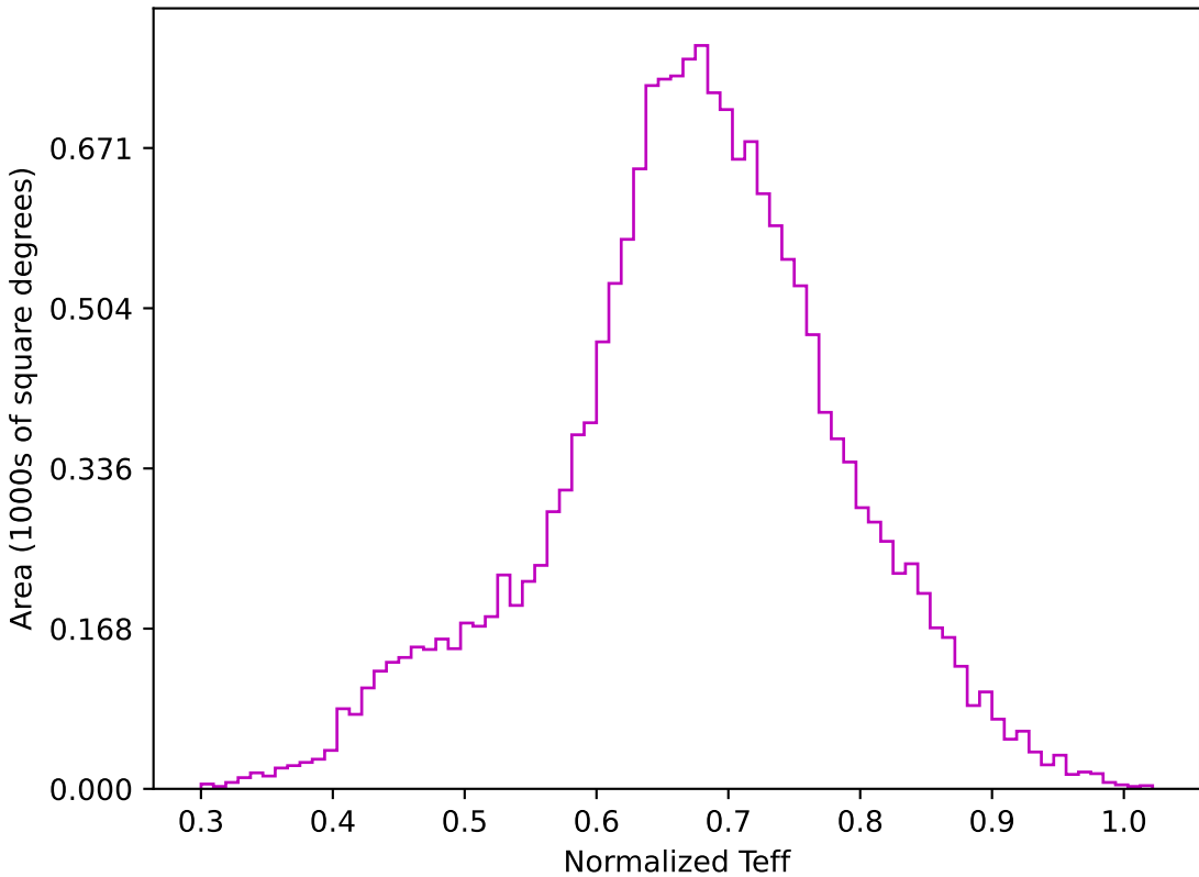
weather_cloudso10v3.4_10yrs WFD z band: Normalized Teff
